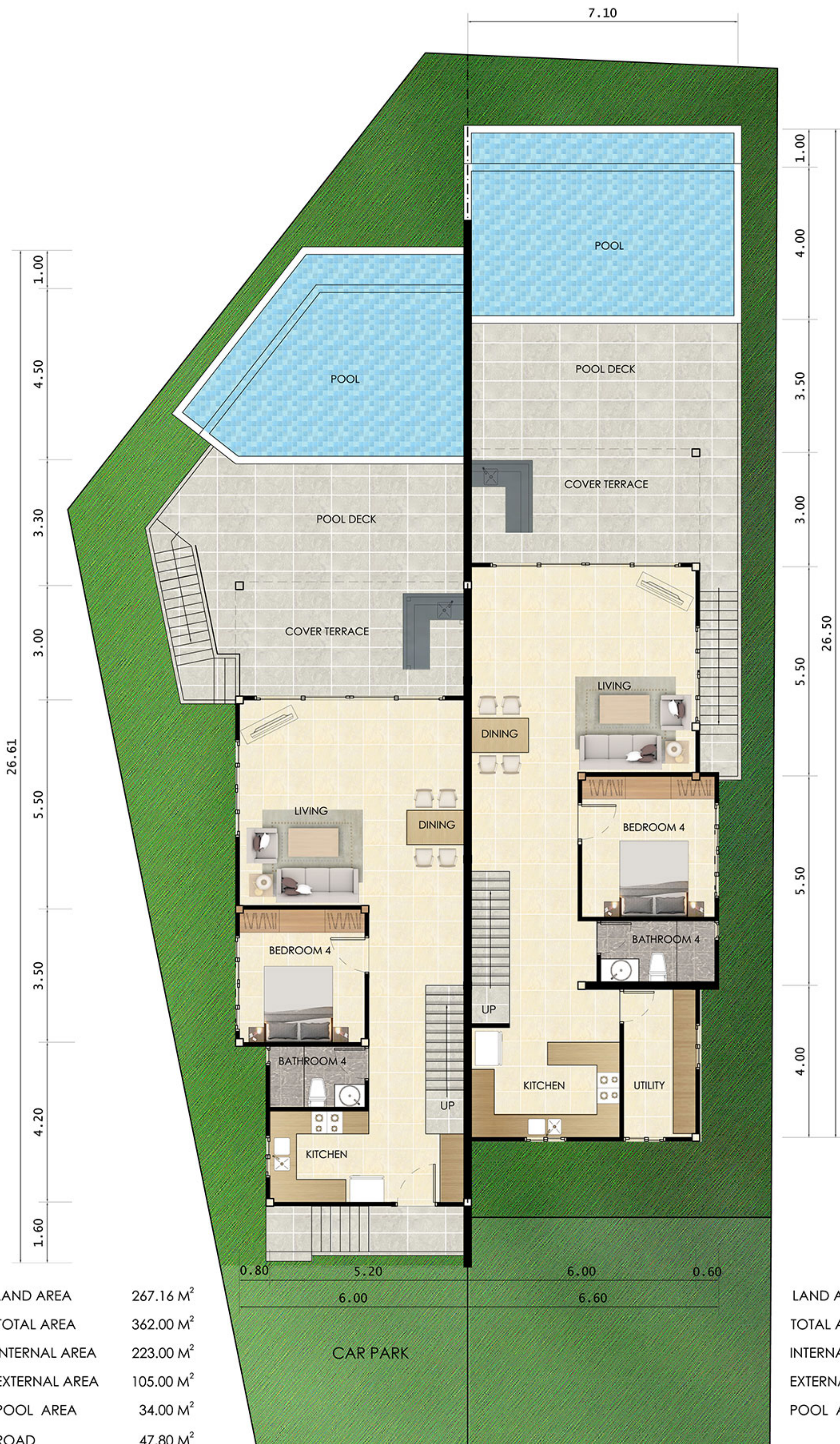
PLOT 5 PLOT 6 GROUND FLOOR PLAN
